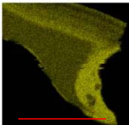
Figure 2: X-ray map showing SiO 2 distribution in KW. The coating is SiO 2 -rich (bright area to right), similar to all the coatings in this study. This coating also contains S. Scale bar is 100 microns.
